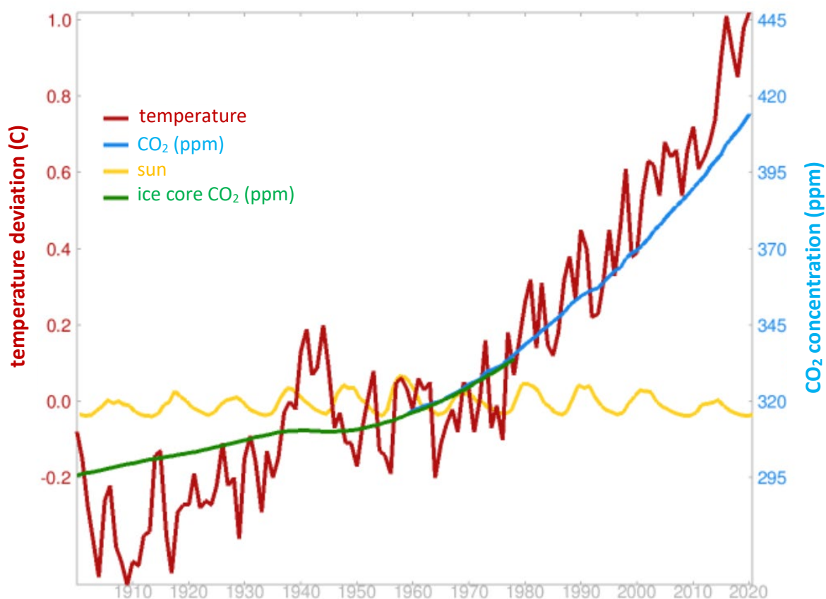
Figure 35: Development of atmospheric CO 2 concentration, mean global temperature change and solar activity ( http://herdsoft.com/climate/widget/ ).
