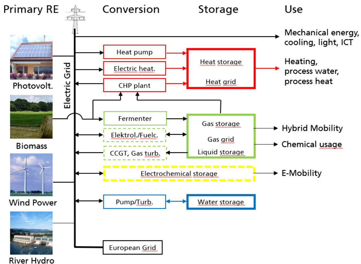
Figure 56: Simplified schematic representation of a renewable energy system with the most important electricity grid-related components of generation, conversion, storage, and consumption; ICT: information and communication technology, CHP: combined heat and power, CCGT: combined cycle gas and steam power plant.
