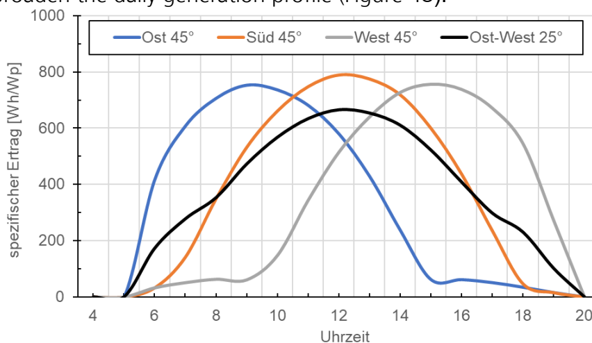
Figure 48: Electricity yield profiles of PV systems mounted in various ways on a predominantly sunny day in May, no shade, located in Freiburg, calculated online using https://re.jrc.ec.europa.eu/pvg_tools .
