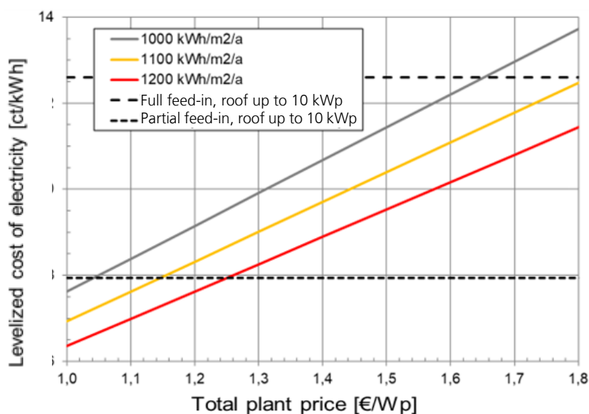
Figure 12: Estimation of the LCOE for small PV systems under different irradiation conditions, plus fixed remuneration according to EEG.
