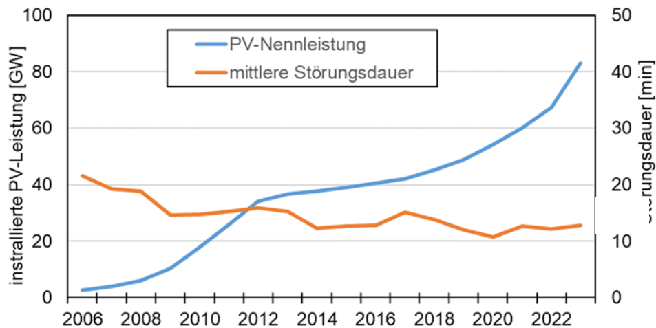
Figure 23: System Average Interruption Duration Index (SAIDI) for low and medium voltage grid. Data from [BNA2].
