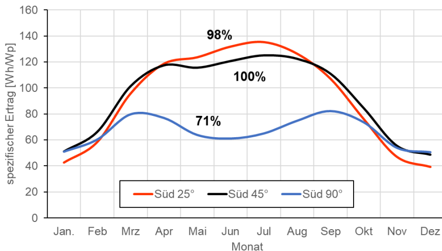
Figure 49: Electricity yield profiles of PV systems mounted in various ways, no shade, located in Freiburg, calculated online using https://re.jrc.ec.europa.eu/pvg_tools ; the percentages provide the relative annual yield in relation to the 45° inclination.
