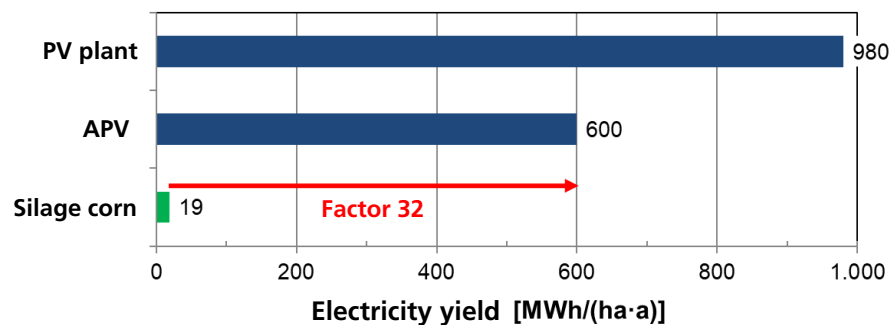
Figure 31: Electricity yields of PV power plants and silage maize per hectare of land used.
