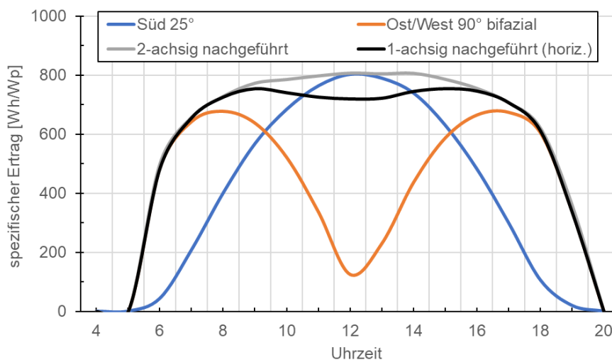
Figure 47: Electricity yield profiles of PV power plants in different mounting variants, calculated online with https://re.jrc.ec.europa.eu/pvg_tools for a predominantly clear day in May at the Freiburg site, no shading, bifaciality factor 100 %.
