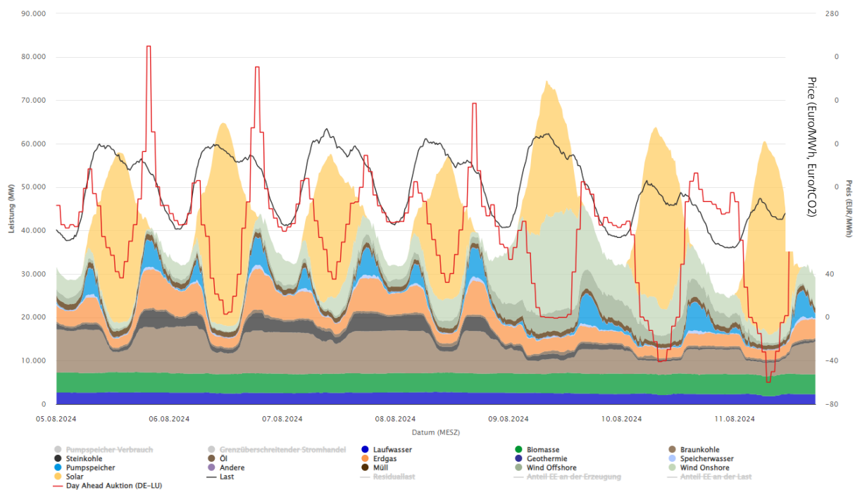
Figure 22: Example showing the course of electricity trading price, conventional and renewable electricity in the 32th calendar week in 2024 [ISE 4].
