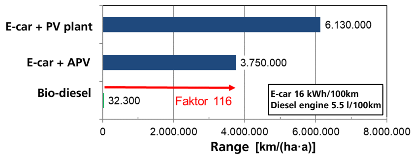
Figure 30: Range of electric and biodiesel vehicles per hectare of land used.
