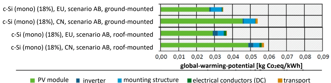
Figure 37: Global warming potential of electricity generation with mono c-Si PV for roof-mounted and ground-mounted systems [UBA7].
