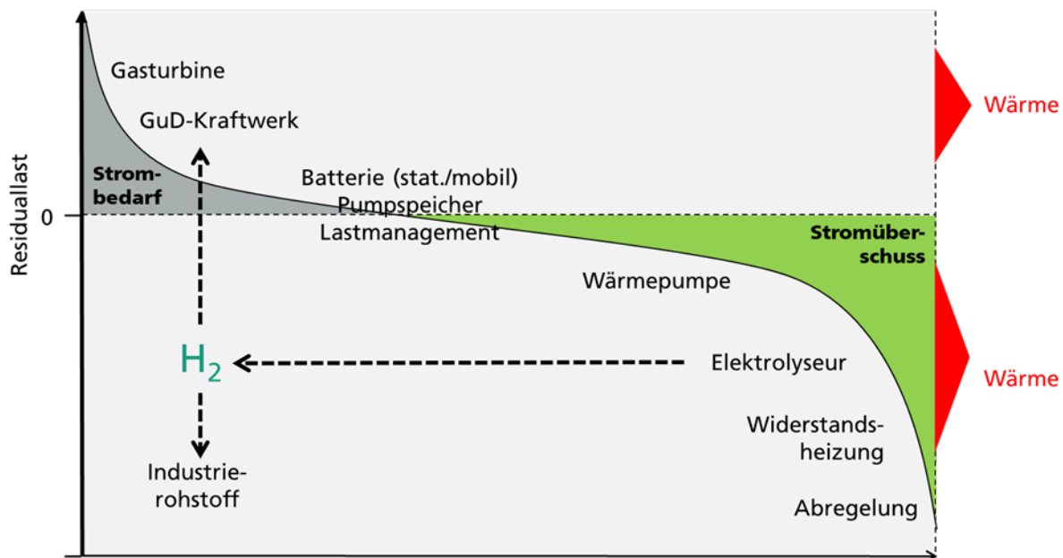
Figure 45: Schematic representation of a residual load curve for Germany with electricity supply with 100 percent RE.
