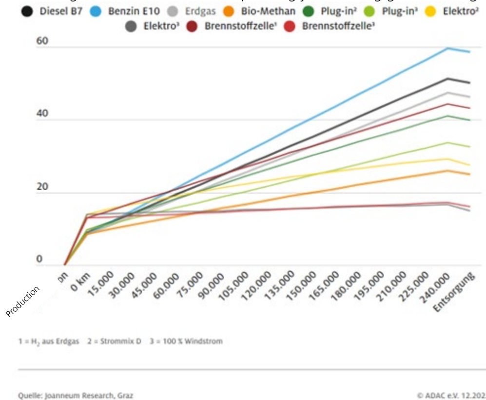
Figure 50: Greenhouse gas emissions (CO 2 -Eq. in tons) of an average compact car with different drives in 2022, in relation to the total mileage [ADAC].
