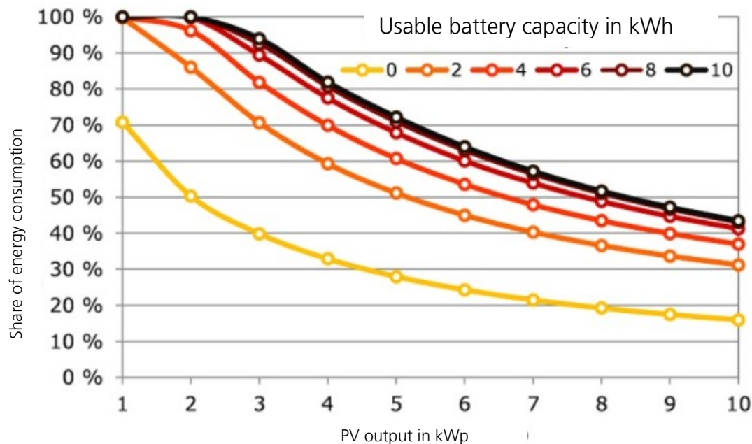
Figure 51: Self-consumption share as a function of battery capacity and power of the solar generator for a single-family household with an annual electricity consumption of 4,700 kWh. [Quasch].
