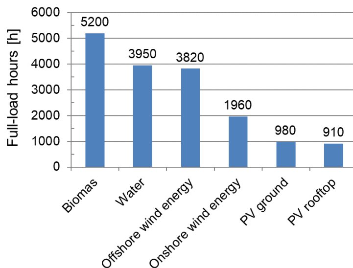
Figure 33: Forecast full utilization hours for electricity generation from EE, data from [ÜNB1].
