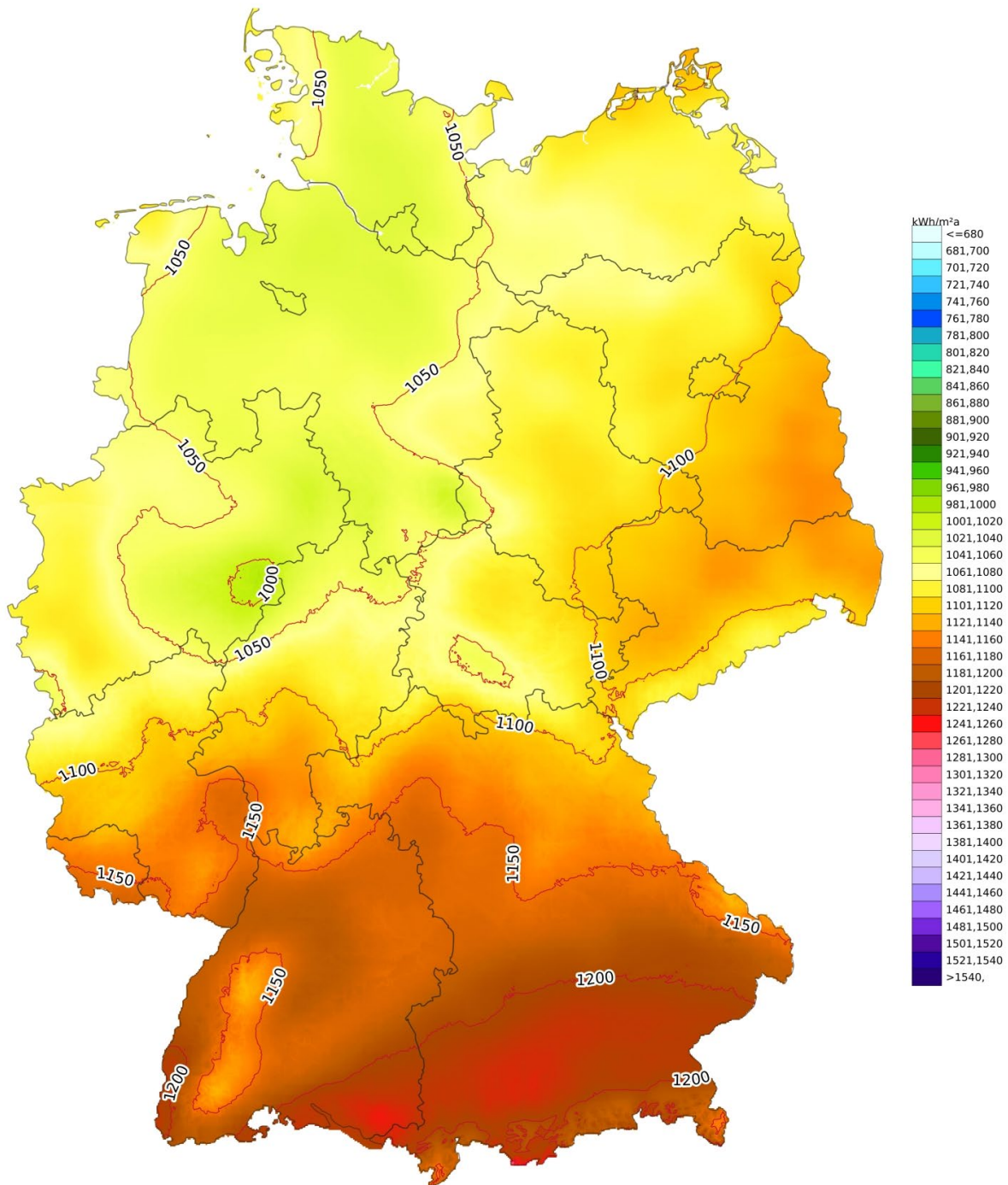
Figure 34: Horizontal annual global radiation total in Germany, averaged over the period 2001-2020 [DWD].
