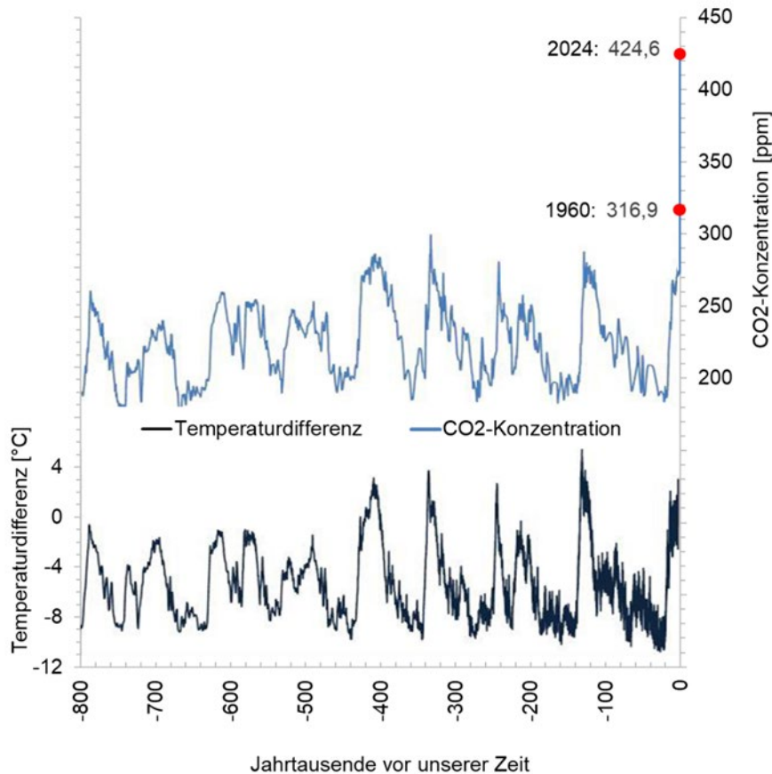
Figure 36: Estimates of atmospheric CO 2 concentration and temperature difference in Antarctica based on ice cores [EPA]; red: CO 2 measurements from Mauna Loa Observatory [ https://www.esrl.noaa.gov/gmd/ccgg/trends/data.html ].
