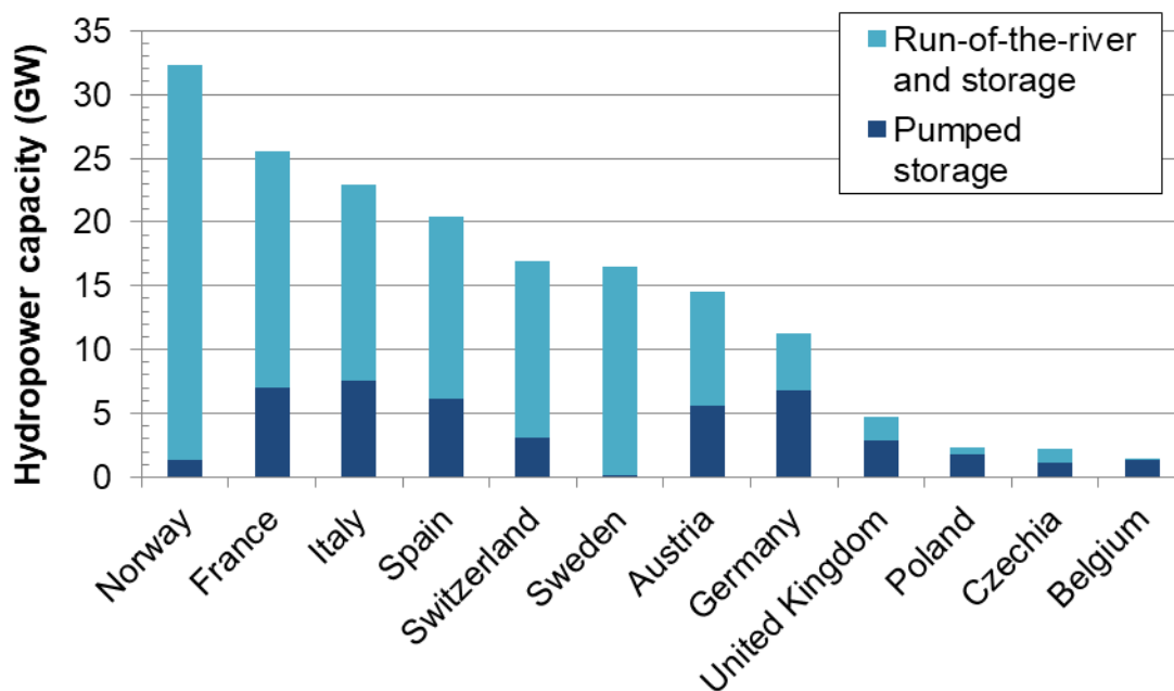
Figure 55: Installed capacity of hydropower plants in neighboring countries, figures from [IHA].
