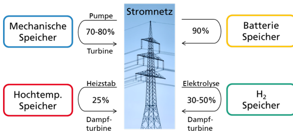
Figure 53: Technologies for the storage of electrical energy at efficiencies achievable today.
