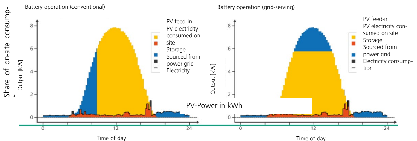
Figure 52: Comparison of conventional and grid-serving operation [ISE7].
