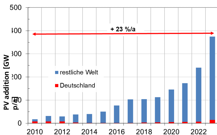
Figure 40: Development of annual PV additions [IEA3] and average annual growth rate.
