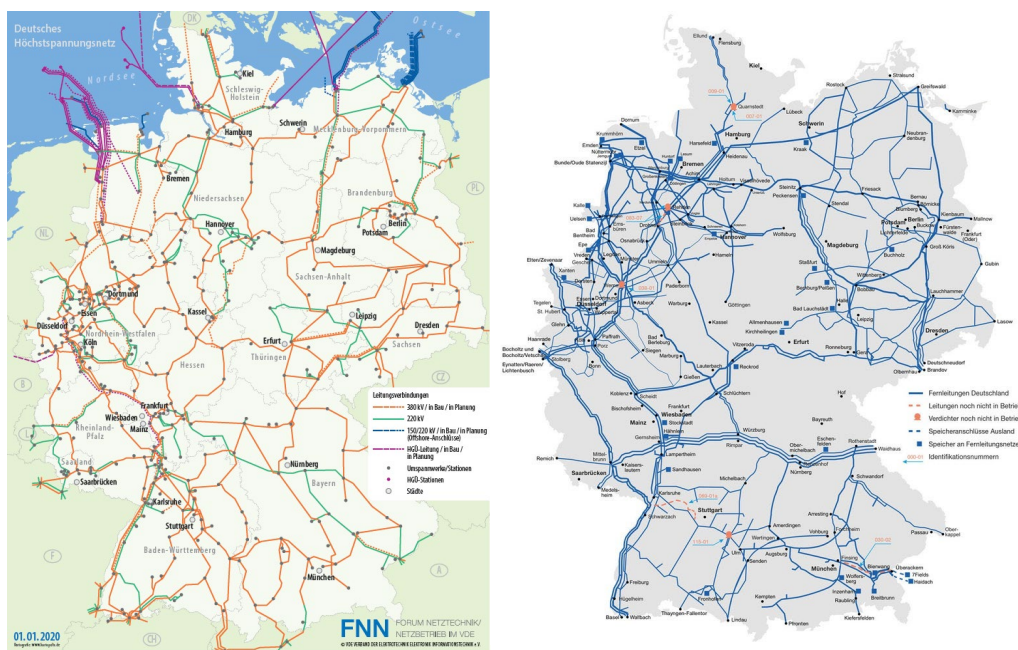
Figure 54: Extra-high voltage grid [VDE] and gas transmission grid [Fern].
