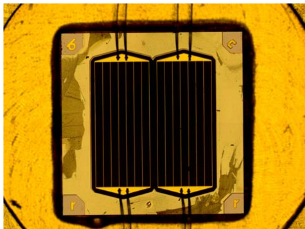
Figure 1: Photo of the new world record solar cell made of \text{Ga}_{0.35}\text{In}_{0.65}\text{P}/\text{Ga}_{0.83}\text{In}_{0.17}\text{As}/\text{Ge} with a cell area of 5.09 mm 2 .
