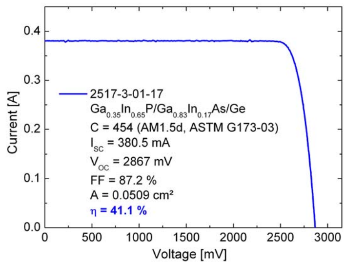
Figure 2: IV characteristics of the GaInP/GaInAs/Ge triple junction solar cell at a solar concentration of 454 suns. The measurements were carried out by the Callab at Fraunhofer ISE.
