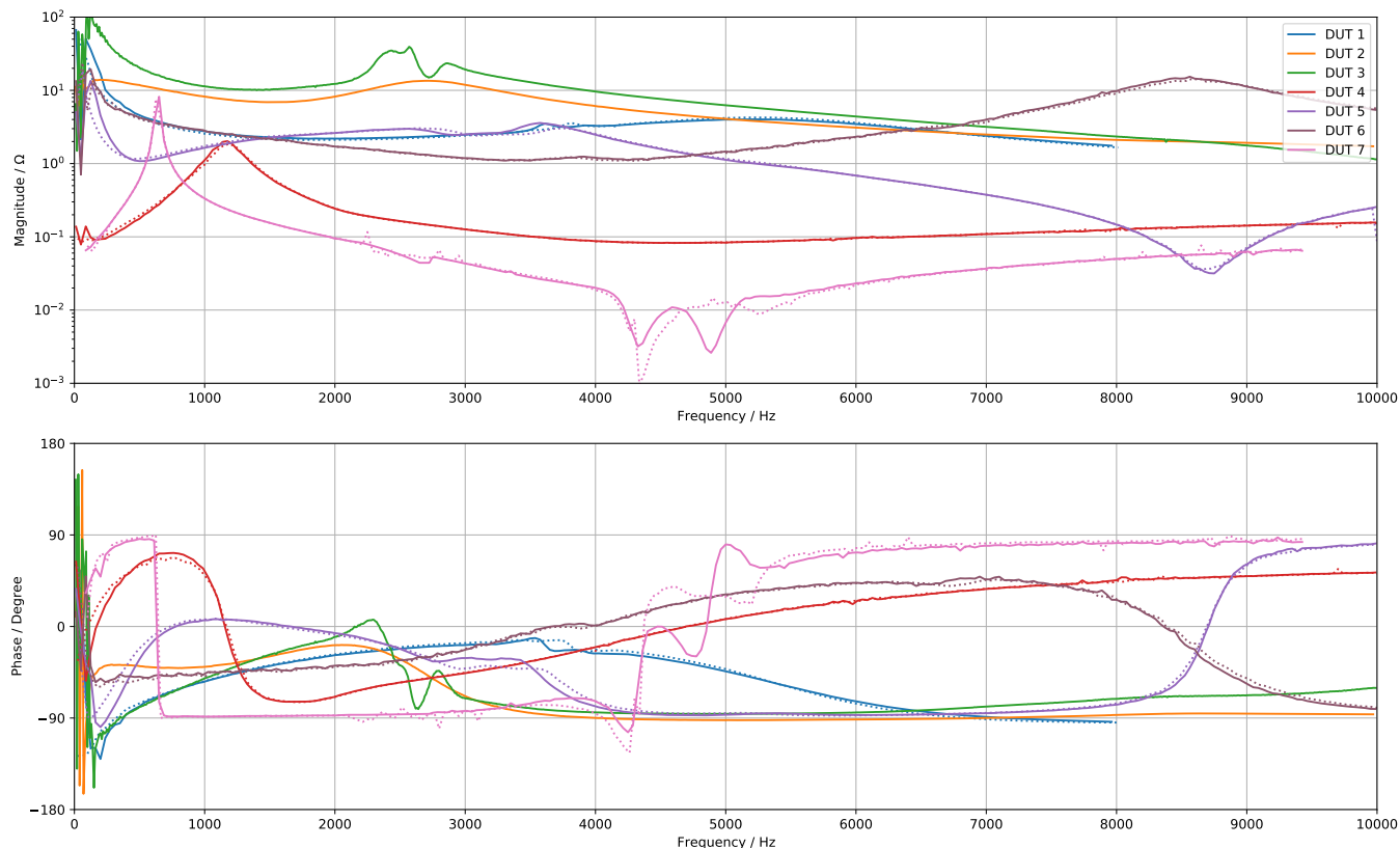
Thévenin Impedance - Positive and Negative Sequence
