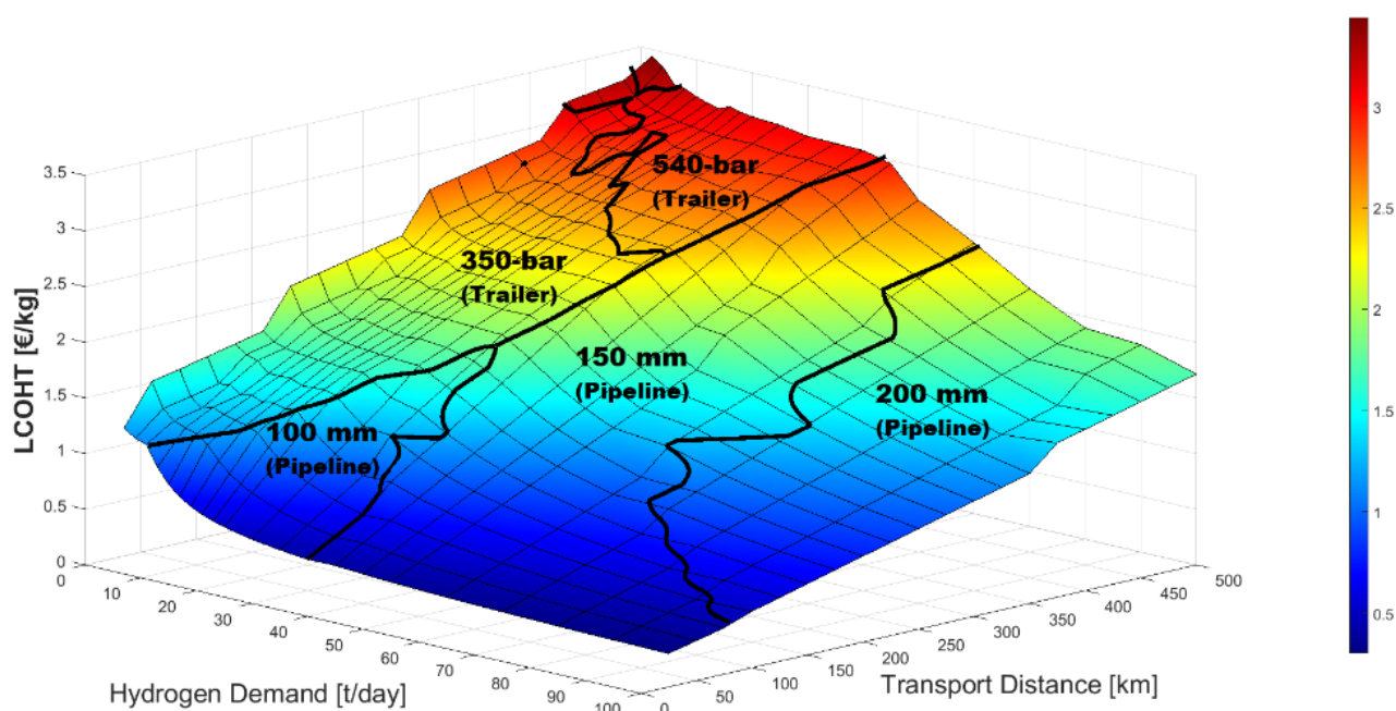
Figure 4.13: Least LCOHT as a function of hydrogen demand and transport distance.
