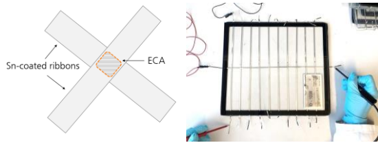
Figure 1: Sample design (left) and measurement (right) for the investigation of the Sn/Ag joint galvanic corrosion.
