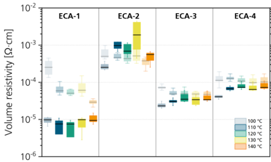
Figure 5: Results of the volume resistivity measurement after curing (transparent) at different temperatures and lamination (full color) of the PCBs. One box plot is represented by 10 measurements. Black lines refer to median values.
