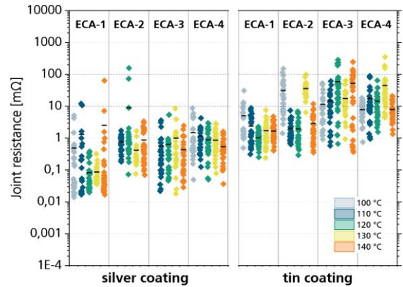
Figure 4: Results of the joint resistance measurement after curing at different temperatures and lamination of the PCBs. Per group, 19 to 57 measurements were performed. One datapoint represents one measurement.
