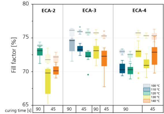
Figure 6: Fill factor of the small-scale modules measured after lamination (transparent) and aTC200 (full color). One box plot is represented by 10 samples. Black lines refer to median values.
