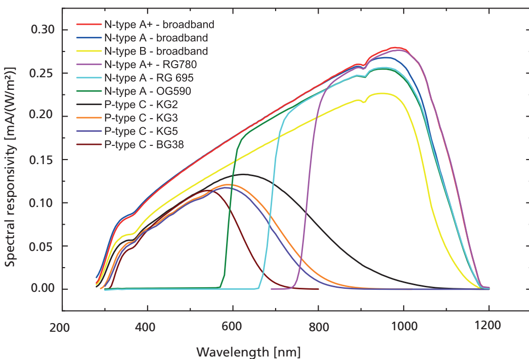
5 Spectral response of different cell type-filter-combinations for reference cells.
